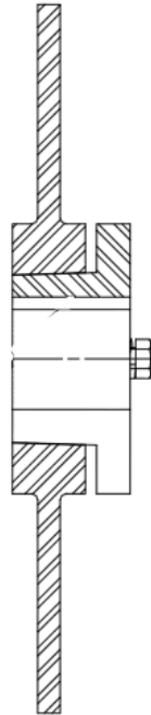
TUSA Doc – (T-1001) Sure-Grip Bushing & Rotor Assembly (Taper lock with disc, QD)
